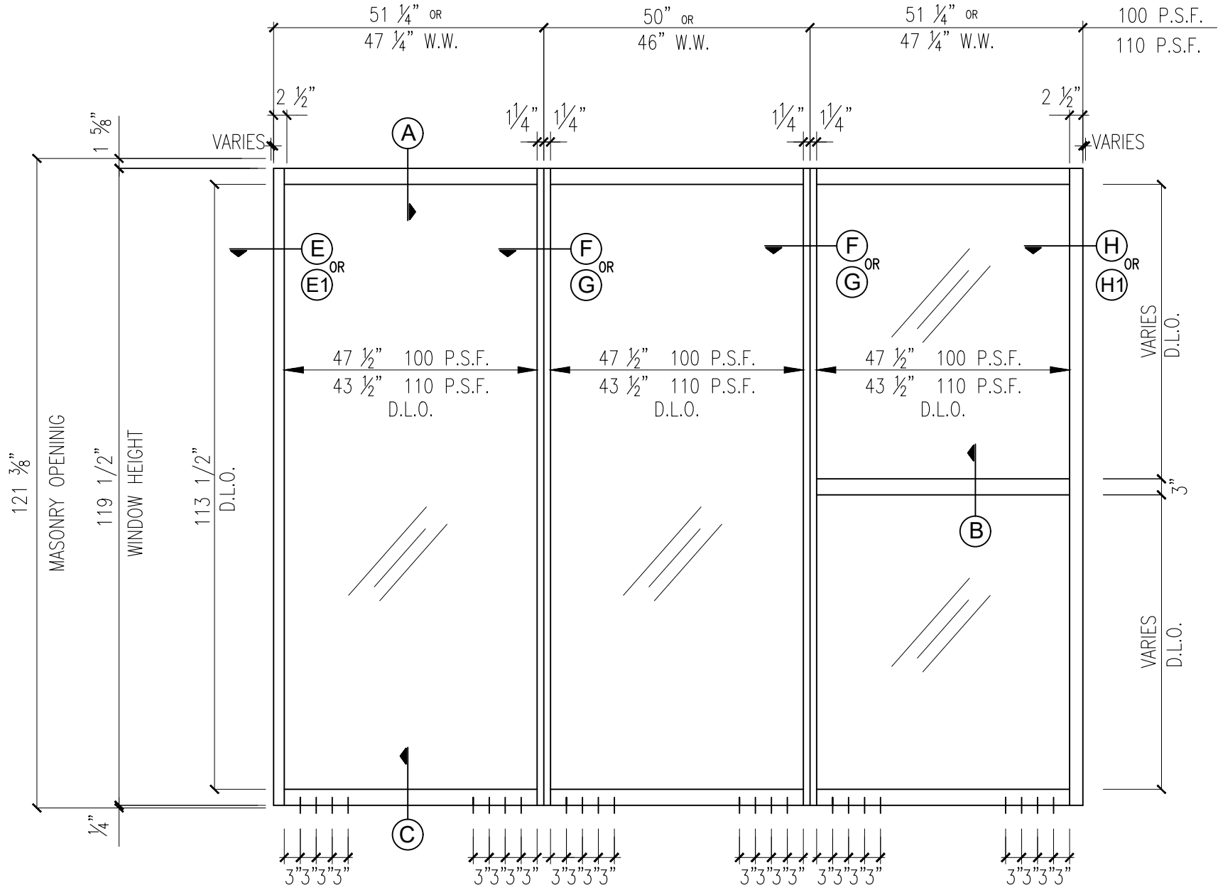
FIXED WINDOW ELEVATION EXTERIOR VIEW
