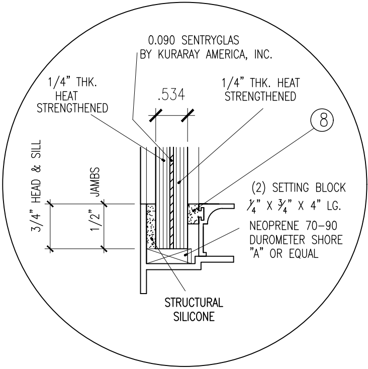
GLAZING DETAIL
