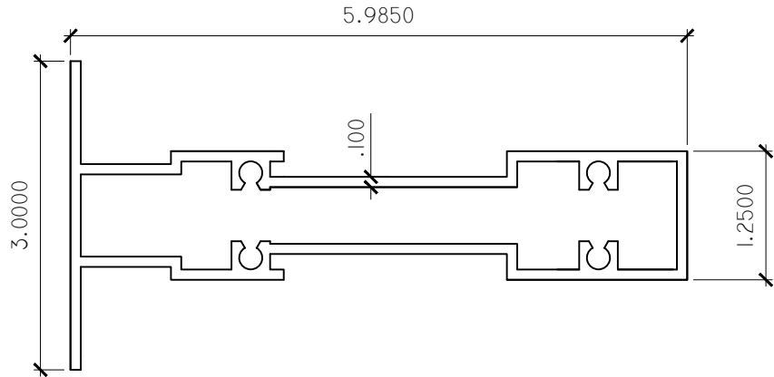
INTERMEDIATE
