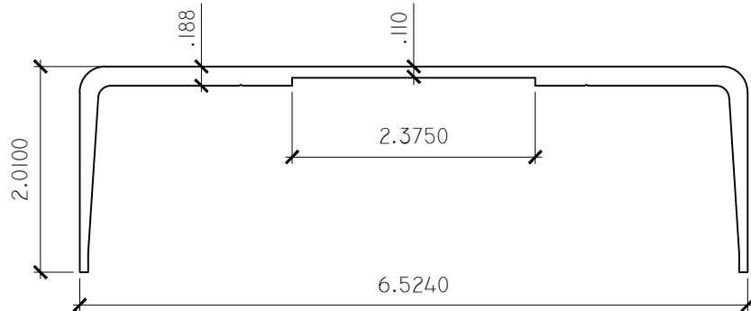
REINFORCING
