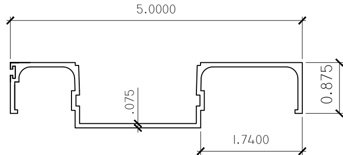
BEAD
